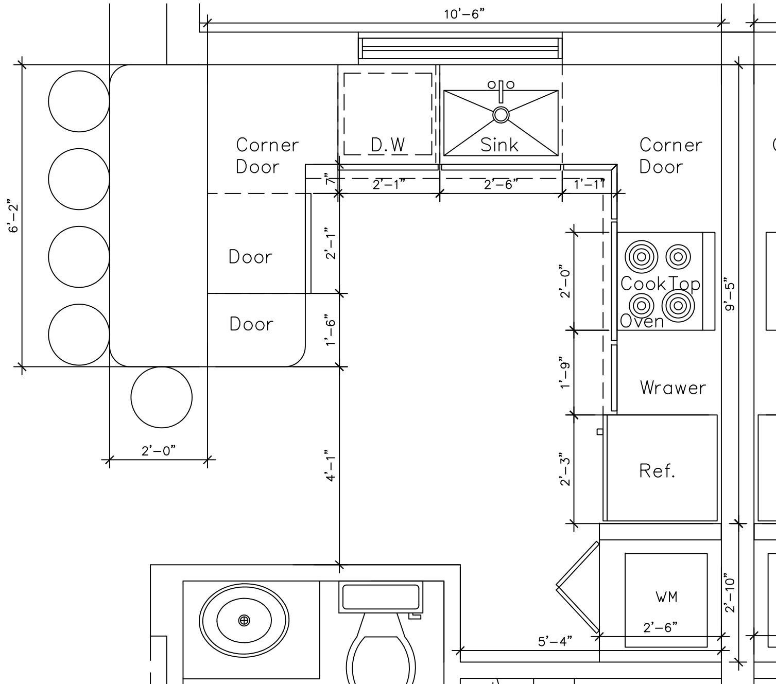
KITCHEN DET
