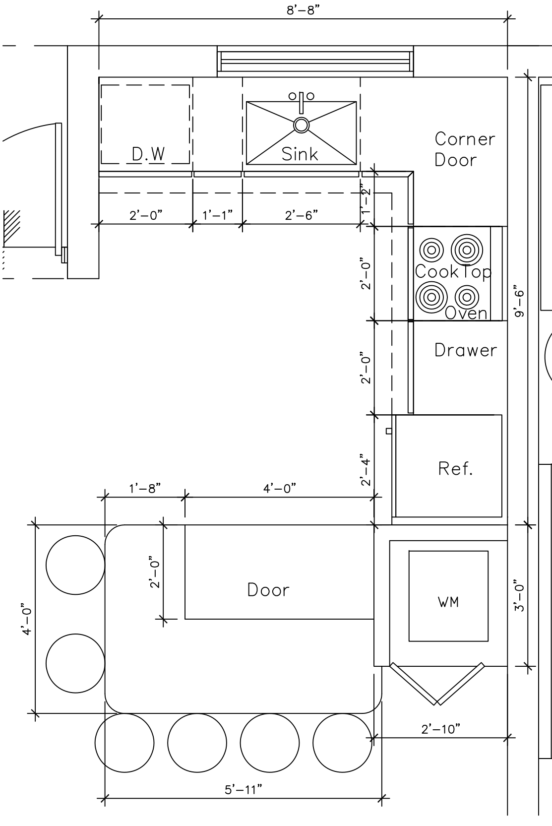
KITCHEN DET
