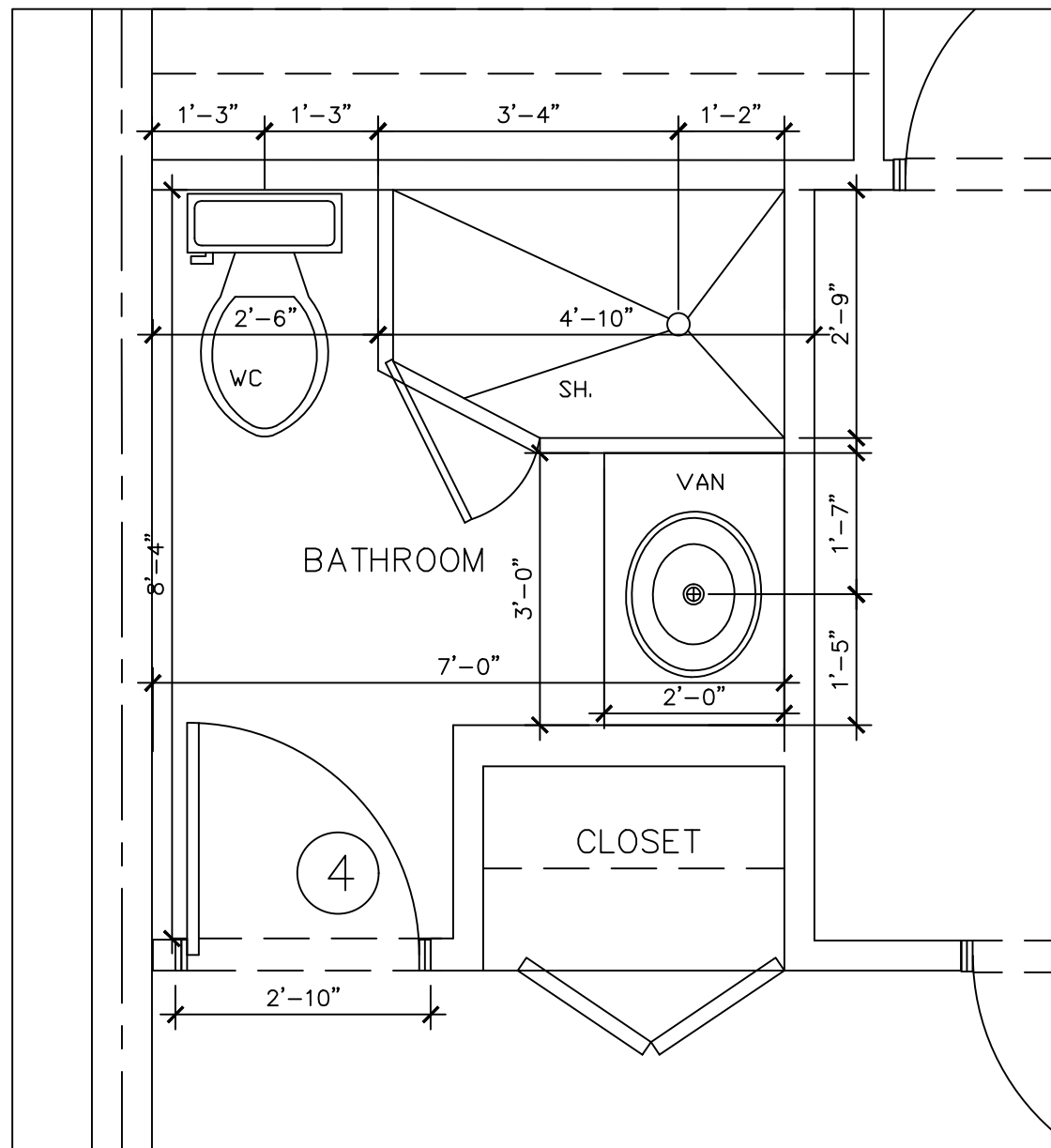
PWDR ROOM DET 5 SCALE: 1/2" = 1"
