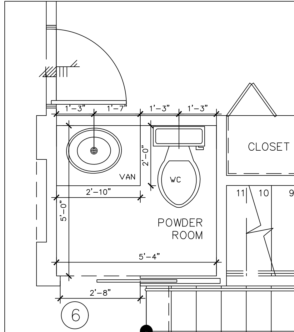
PWDR ROOM DET 2 SCALE: 1/2" = 1"
