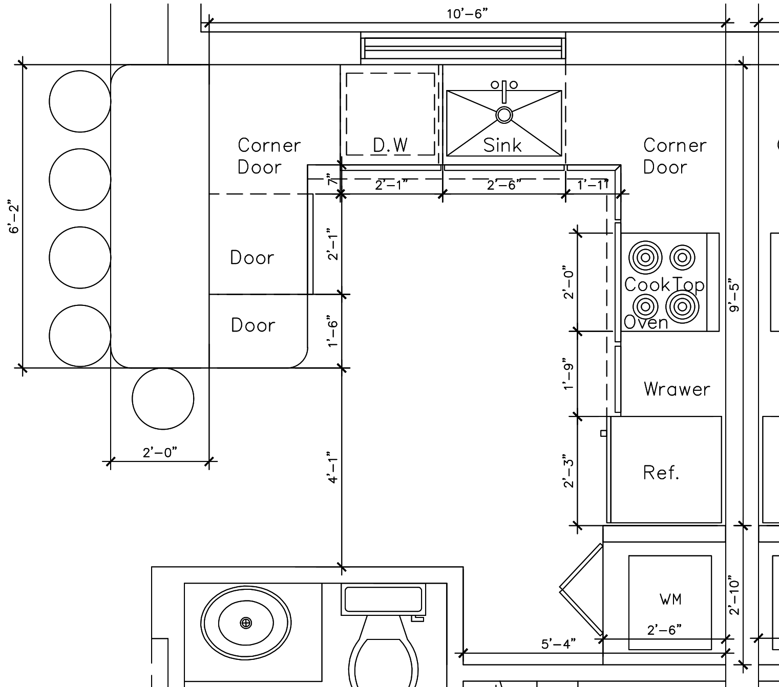
KITCHEN DET 8 SCALE: 1/2" = 1"
