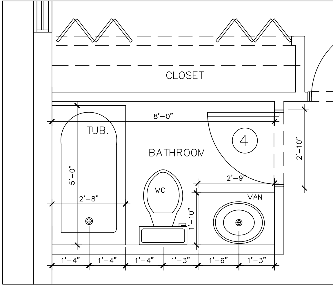
PWDR ROOM DET 3 SCALE: 1/2" = 1"
