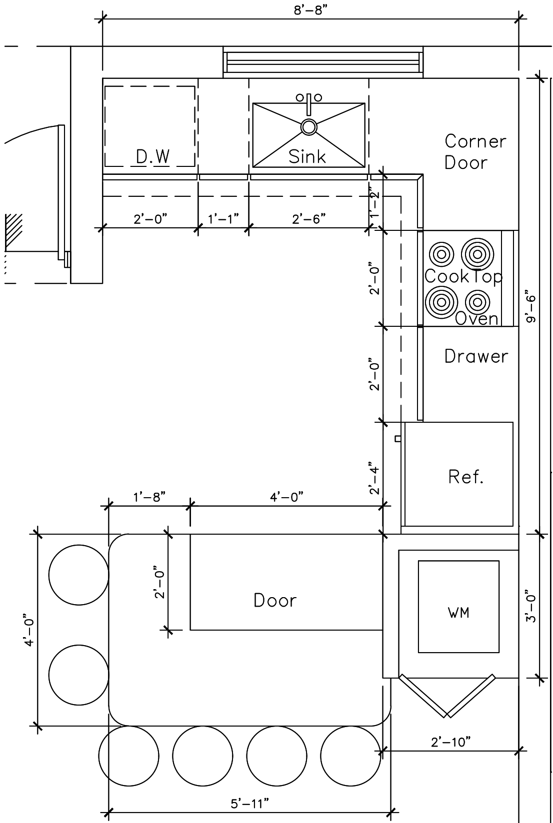
KITCHEN DET 7 SCALE: 1/2" = 1"
