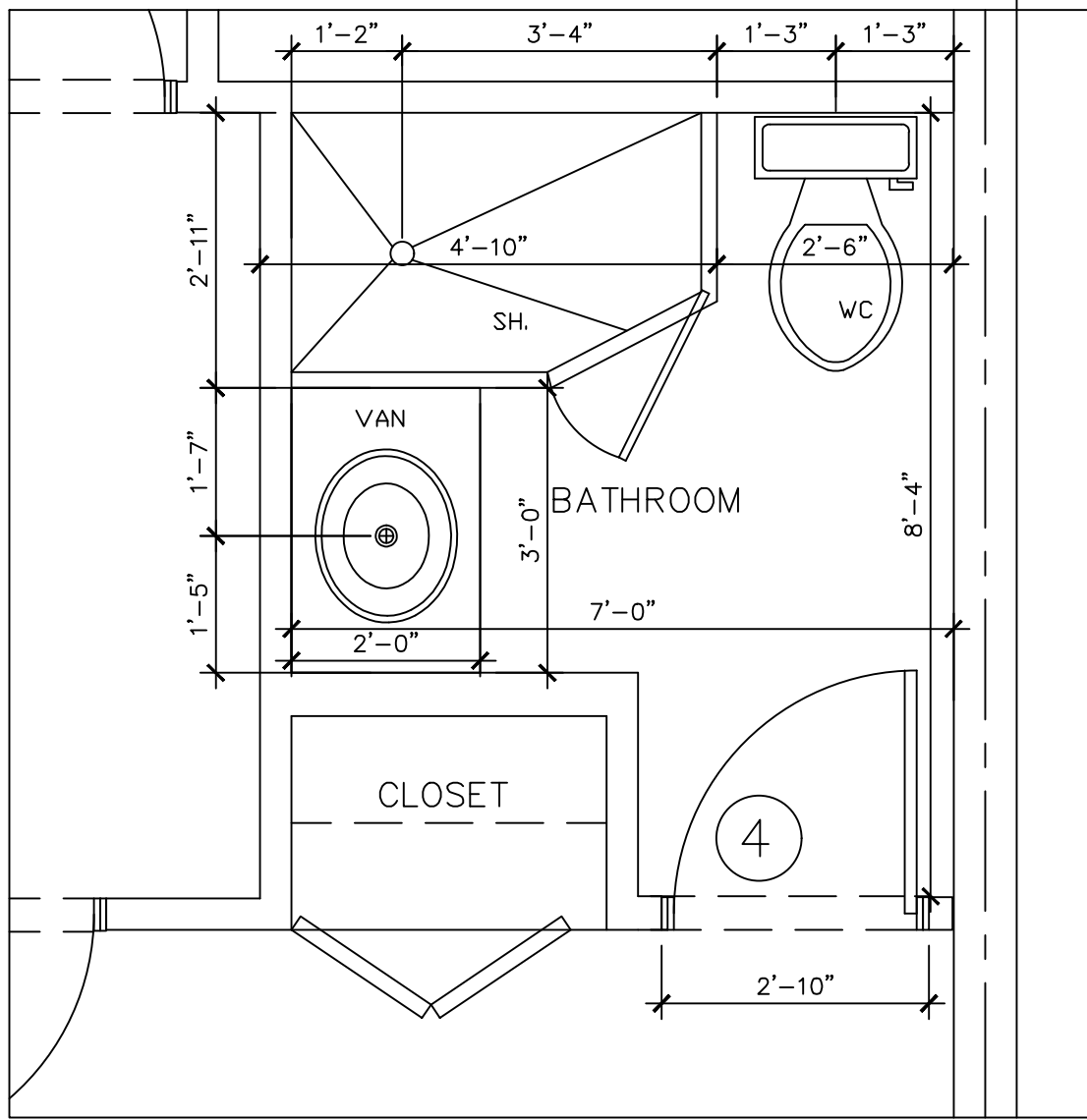
PWDR ROOM DET 4 SCALE: 1/2" = 1"
