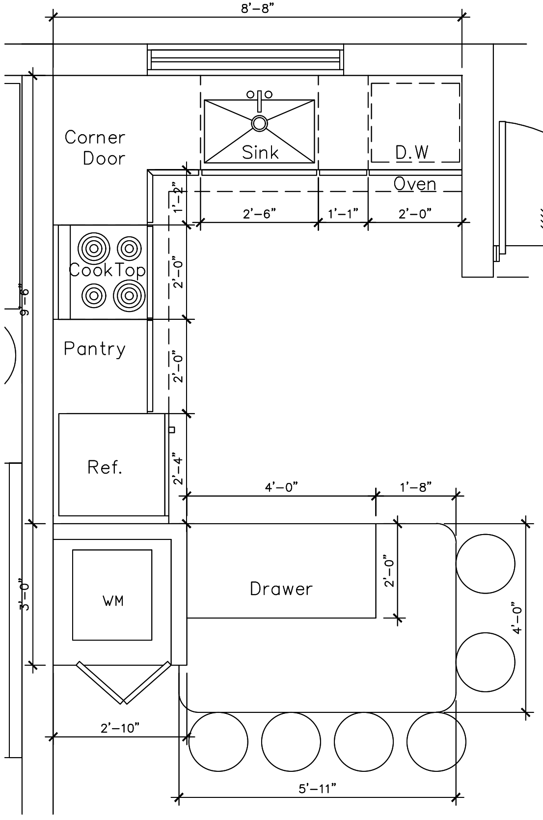
KITCHEN DET 10 SCALE: 1/2" = 1"
