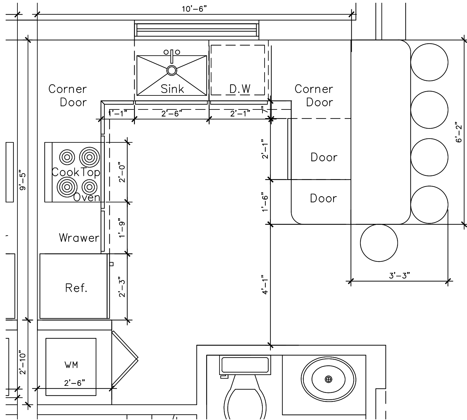
KITCHEN DET 9 SCALE: 1/2" = 1"
