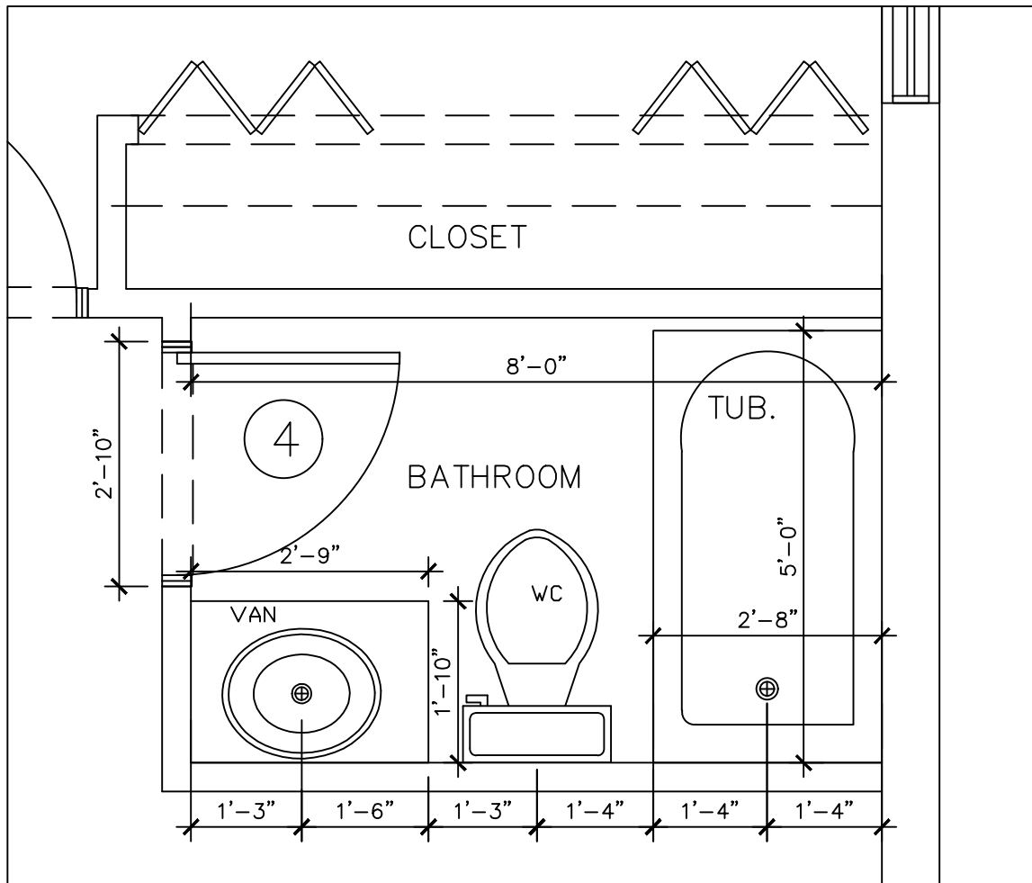
PWDR ROOM DET 6 SCALE: 1/2" = 1"
