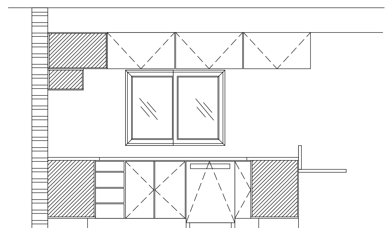
KITCHEN ELEV DET 10 SCALE: 1/2" = 1"
