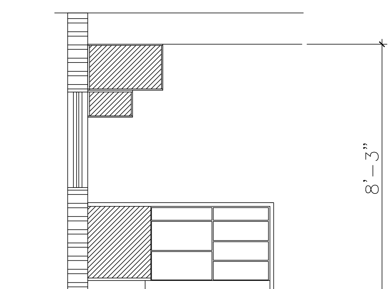
KITCHEN ELEV DET 10 SCALE: 1/2" = 1"
